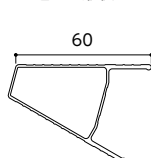
踏ざん形状
