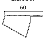
踏ざん形状
